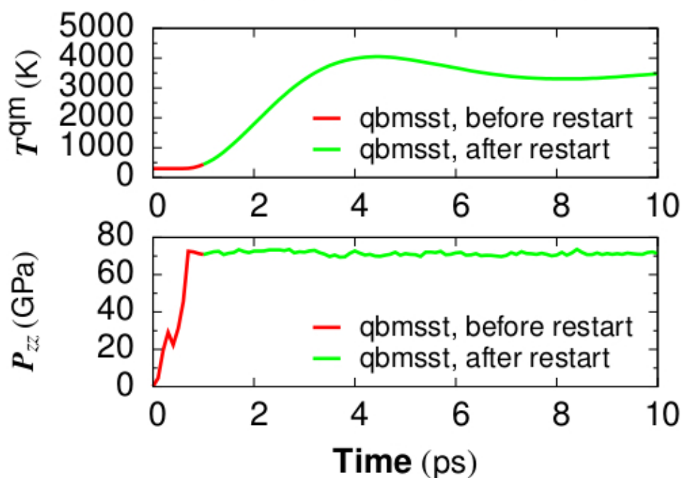
Figure 2. Quantum temperature and pressure vs. time for simulating shocked alpha quartz with the QBMSST. The shock propagates along the z direction. Restart of the QBMSST command is demonstrated in the example input script. Thermodynamic quantities stay continuous before and after the restart.
