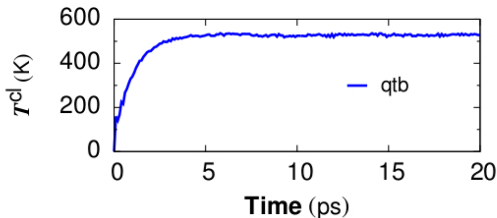
Figure 1. Classical temperature T^{\text{cl}} = \frac{1}{2} m_i v_i^2 / 3Nk_B vs. time for coupling the alpha quartz initial state with the quantum thermal bath at target quantum temperature T^{\text{qm}} = 300\text{ K} . The NpH ensemble is used for time integration while QTB provides the colored random force. T^{\text{cl}} converges at the timescale of damp which is set to be 1 ps.
